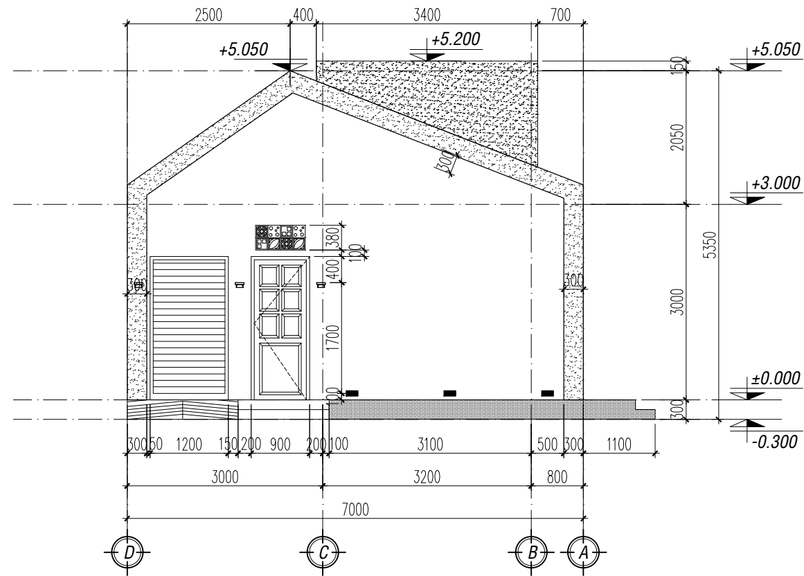
REAR ELEVATION
