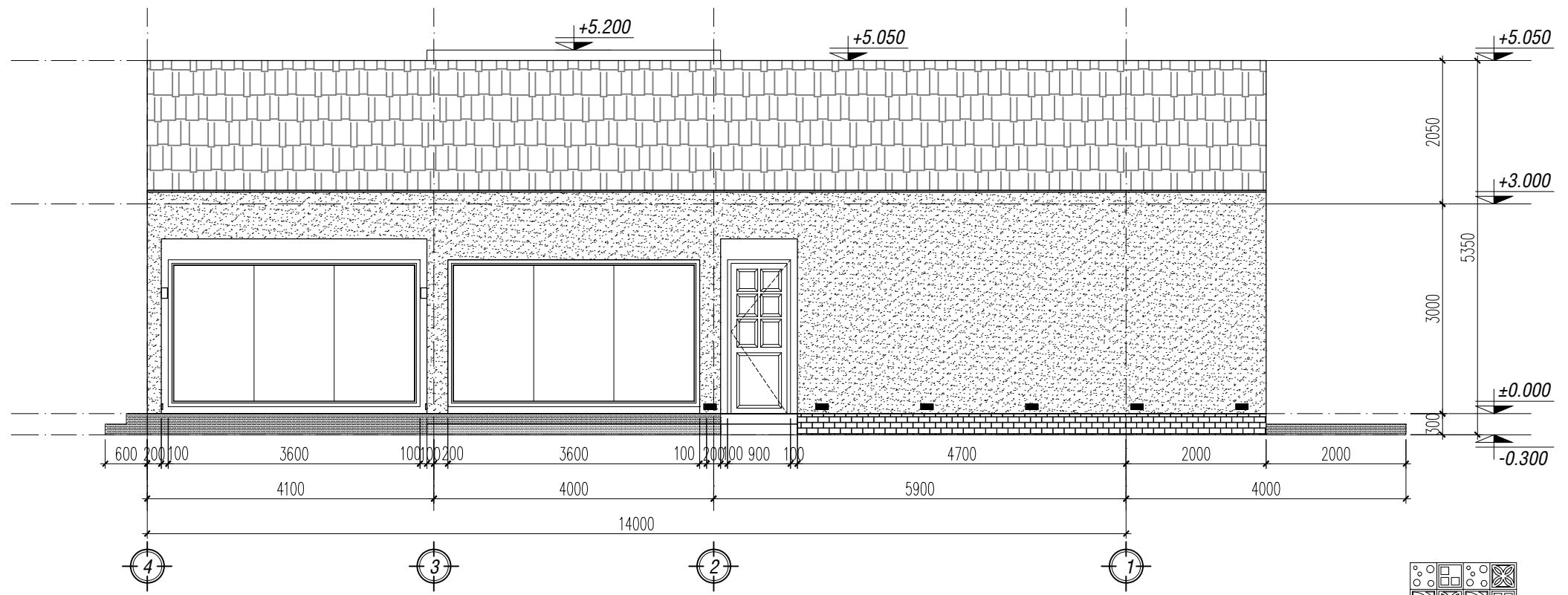
LEFT ELEVATION
