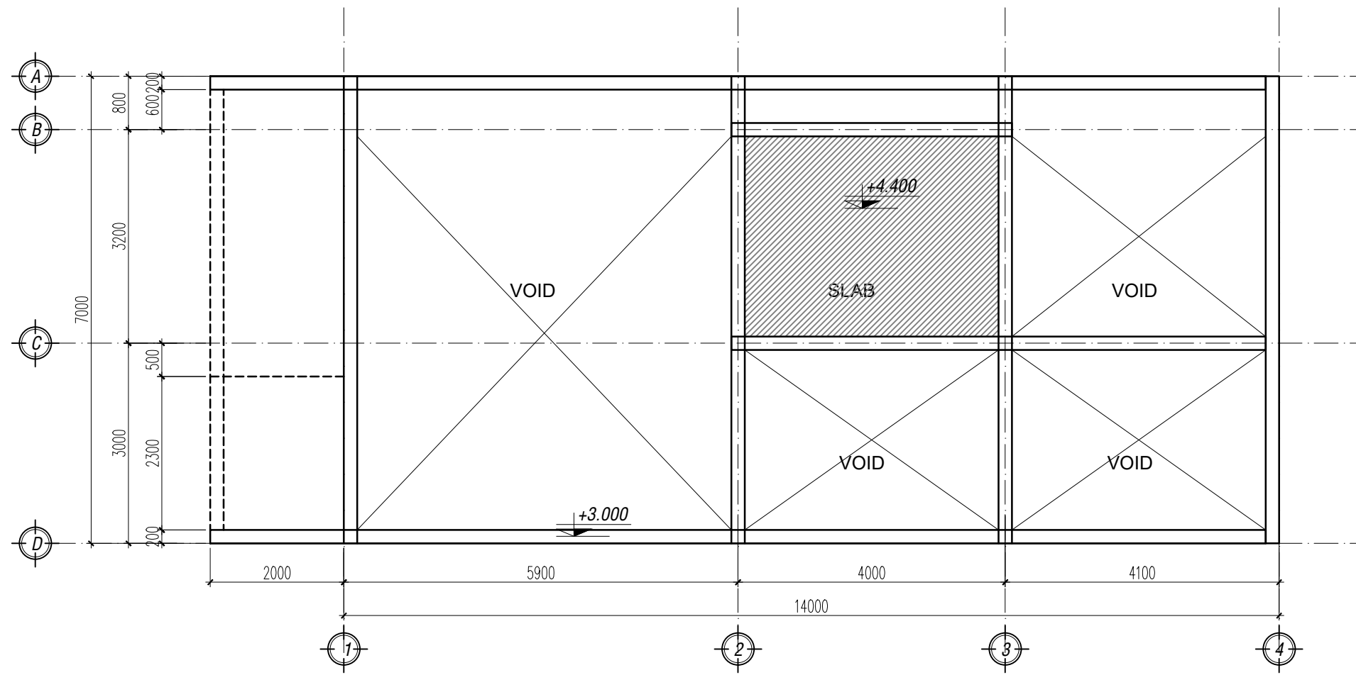
FLOOR PLAN AT +3.400
