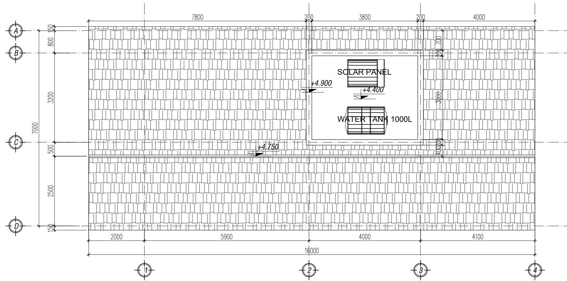
ROOF FLOOR PLAN
